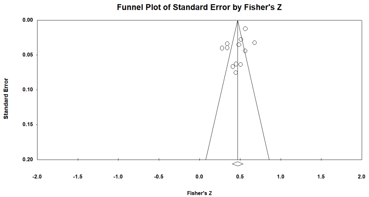
Figure. Funnel plot of Standard Error for Stress and COVID-19
