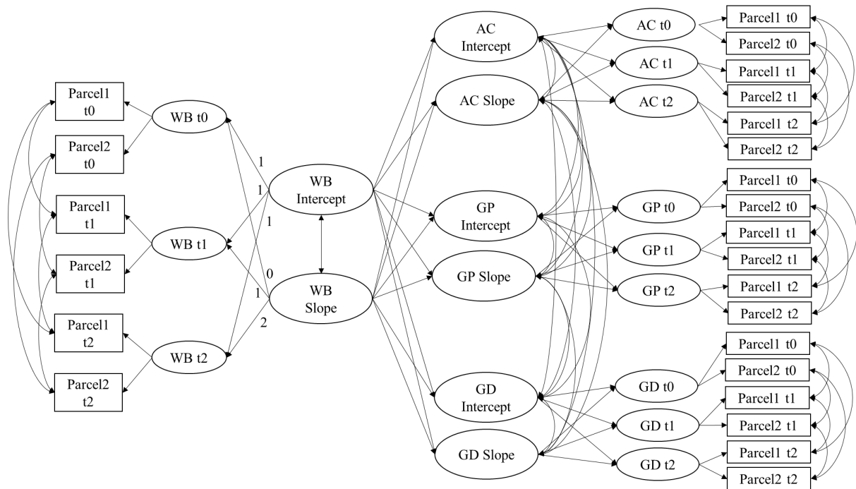
Figure E1: Latent growth model
