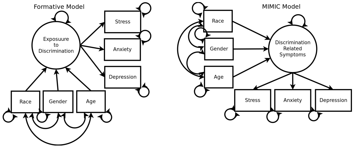
Figure 3: Formative model and MIMIC model for example from Bollen & Lennox, 1991.
