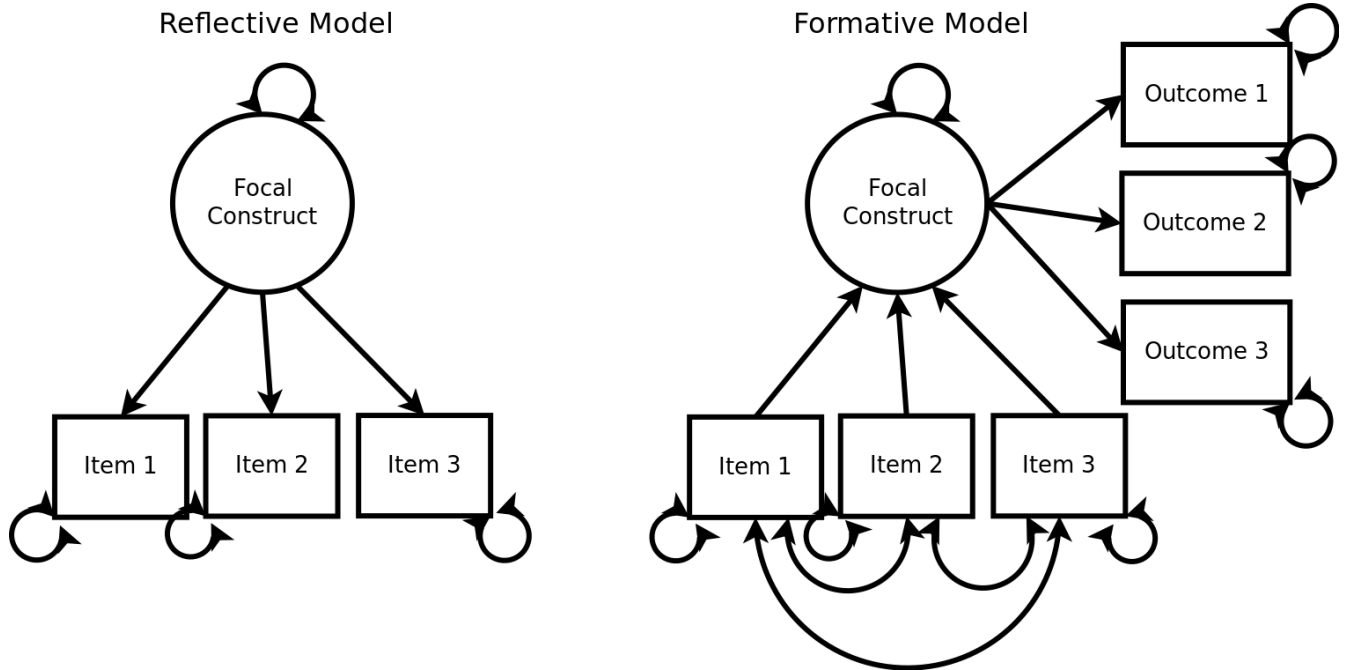
Figure 2: Formative model with a method factor.
