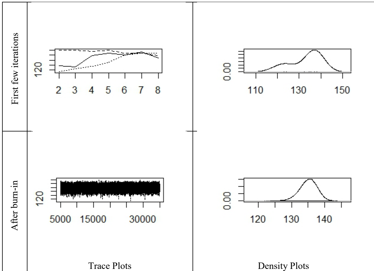
Figure 2E: Trace and Density Plots after 8, and 30,000 iterations and burn-in for three chains
